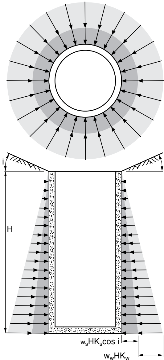
Figure 2 Forces Acting on Manhole
