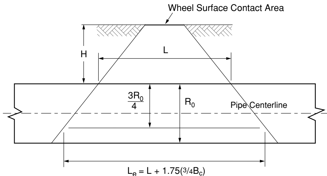
Figure 7 Effective Supporting Length of Pipe
