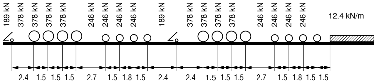
Figure 2 Cooper E 85 Wheel Loads and Axle Spacing
